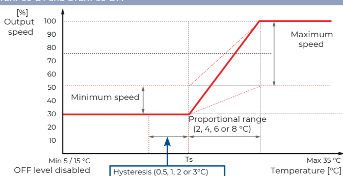
GTEXI-60-DT and GTEXI-60-DM
